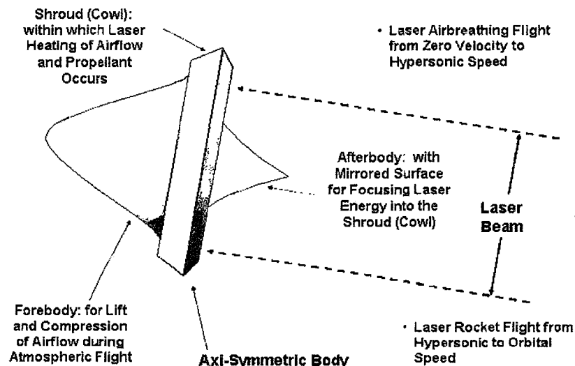
Figure 7. Lightcraft Concept [26].
