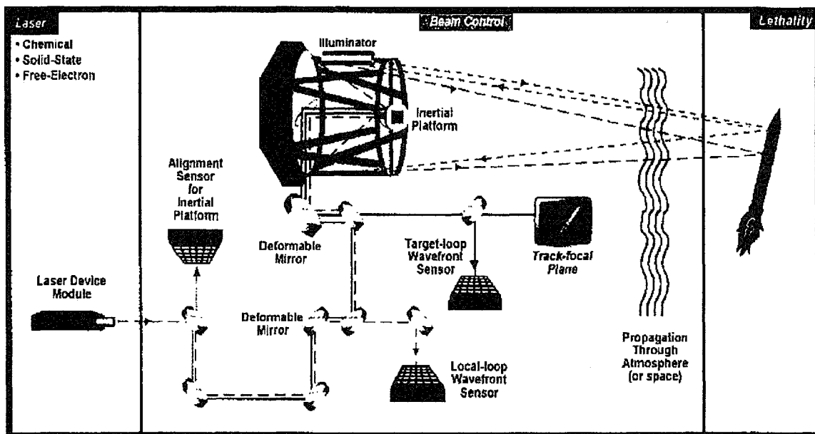
Figure 33. Notional Long Range HEL Beam Control System (courtesy of the Directed Energy Professional Society).
