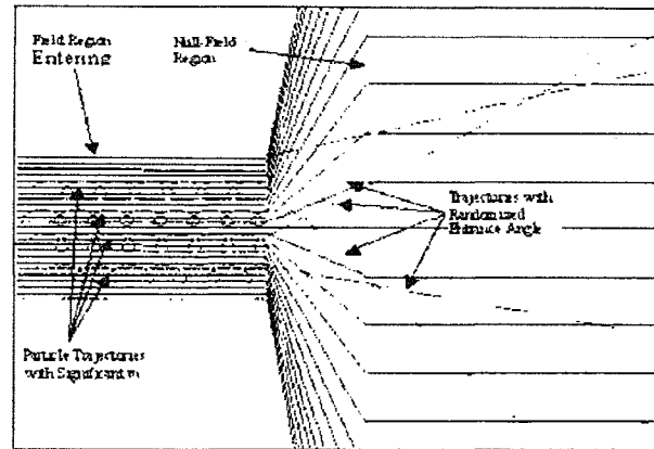
Figure 5.10. Diagram of Direction Randomization (KAM effect) Due to the Magnetic Field Null Region in the IEC
