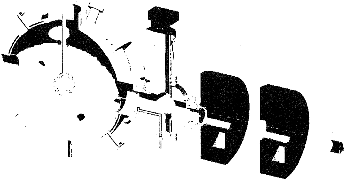
Figure 2.6. ^3\text{He} Ion Source for Use in ^3\text{He}-^3\text{He} Fusion Rate Studies at the U of Wisconsin
