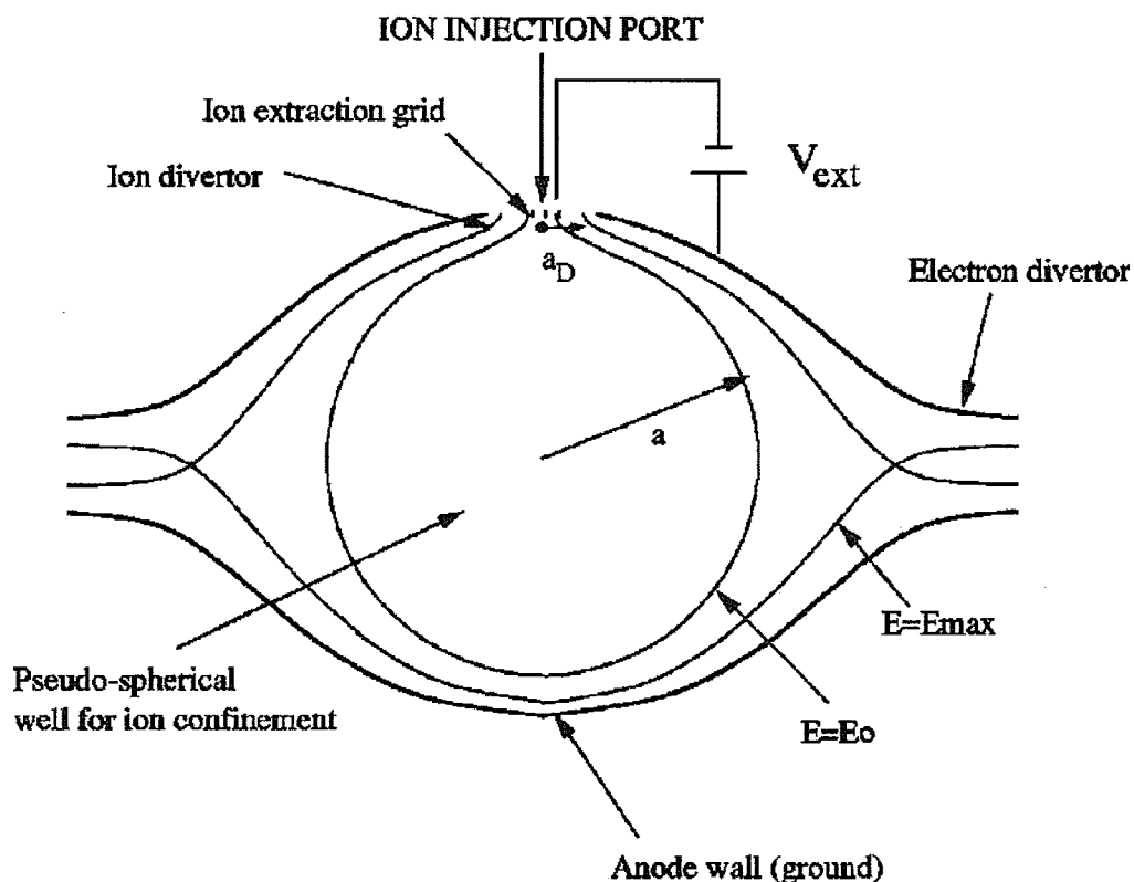
Figure 4.2. Detail of the Anode and the Ion Injection Port in PFX-I (not to scale). Ion and electron divertors are indicated, as well as the E_0 and E_{\max} equipotential lines that define the ion confinement region. The E_0 contour line determines the region of absolute ion confinement.
