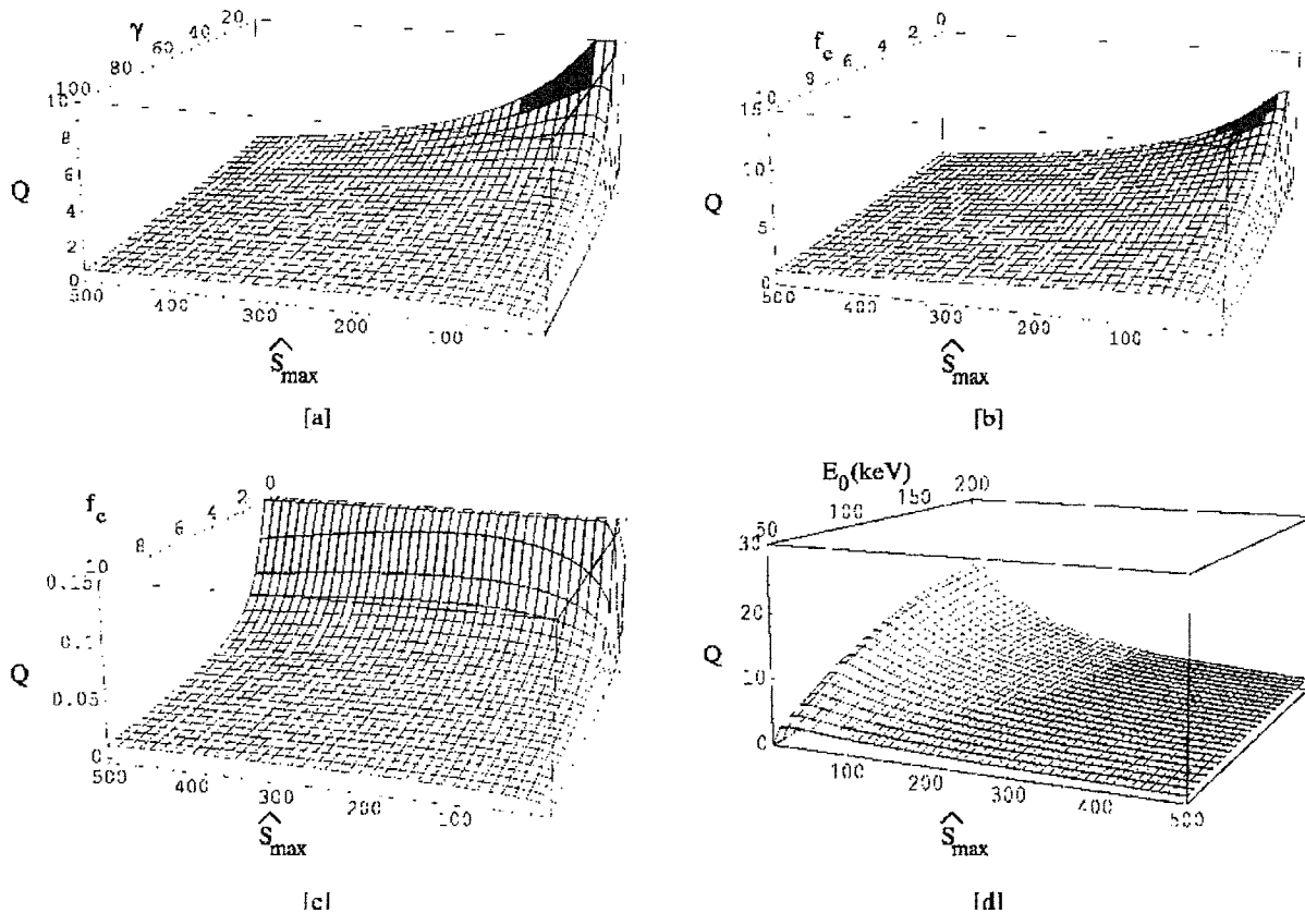
Figure 4.3. Plot of the Q-value (including electron losses) as a function of (a) \hat{S}_{\max} and \gamma with f_e = 10^{-3} , (b) \hat{S}_{\max} and f_e with \gamma = 5 , (c) \hat{S}_{\max} and f_e with \gamma = 100 , and (d) \hat{S}_{\max} and E_0 with \gamma = 5 and f_e = 10^{-3} . These plots have been obtained for E_0 = 100 keV [except (d)], \theta_b = 0.01 , and \bar{E}_s = 1.04 . (Nomenclature is defined in Reference 4.2).
