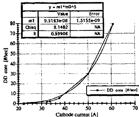
Figure 4.9. The D-D Fusion Reaction Rate Versus Cathode Current for d_{\perp} perp, i = 8\text{keV}
