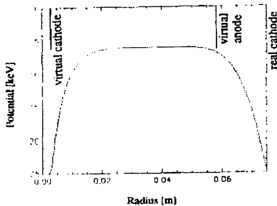
Figure 4.7. The Double Well Potential Calculated With IXL Code for d_{\perp} perp, i=14\text{keV} , I_i=55\text{A} , I_e=59\text{A}
