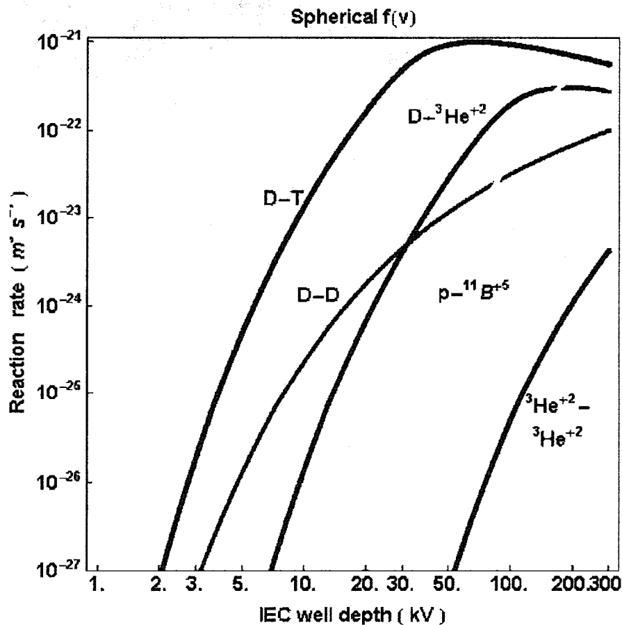
Figure 6.1. p- 11 B Fusion Cross Section Energy Requirements. The p- 11 B reaction rate approaches that of D-T at very high energies, i.e. deep potential wells.
